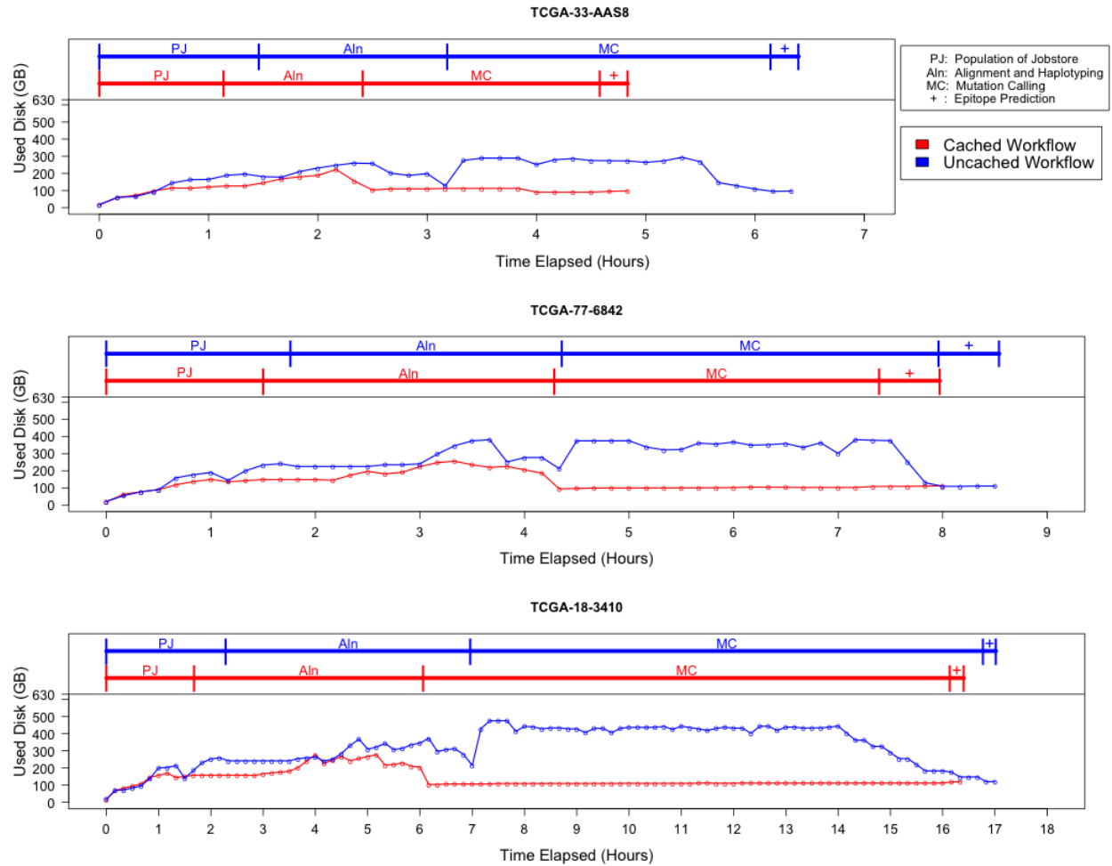
Fig. 3.2: Figure 2: Efficiency gain from caching. The lower half of each plot describes the disk used by the pipeline recorded every 10 minutes over the duration of the pipeline, and the upper half shows the corresponding stage of the pipeline that is being processed. Since jobs requesting the same file shared the same inode, the effective load on the disk is considerably lower than in the uncached case where every job downloads a personal copy of every file it needs. We see that in all cases, the uncached run uses almost 300-400GB more than the cached run in the resource heavy mutation calling step. We also see a benefit in terms of wall time for each stage since we eliminate the time taken for file transfers.
